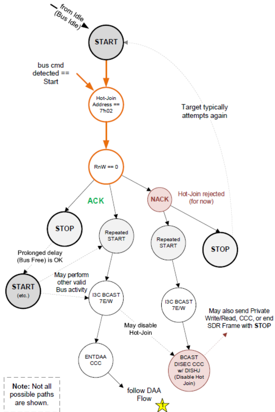
Figure 261 Hot-Join FSM
